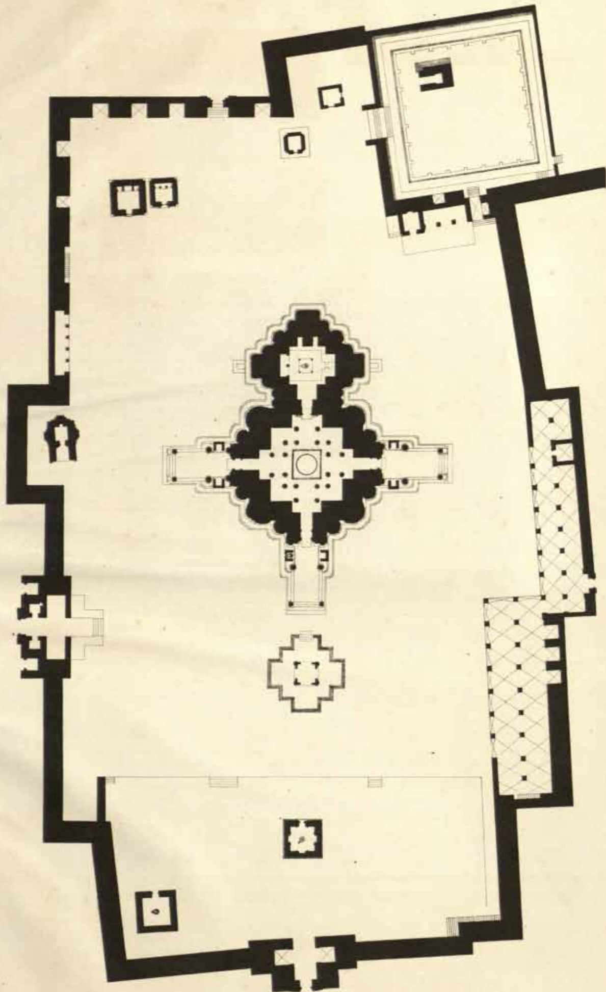
NAGANATHA TEMPLE: AUNDHA (PARBHANI). SCALE 40' TO 1".
