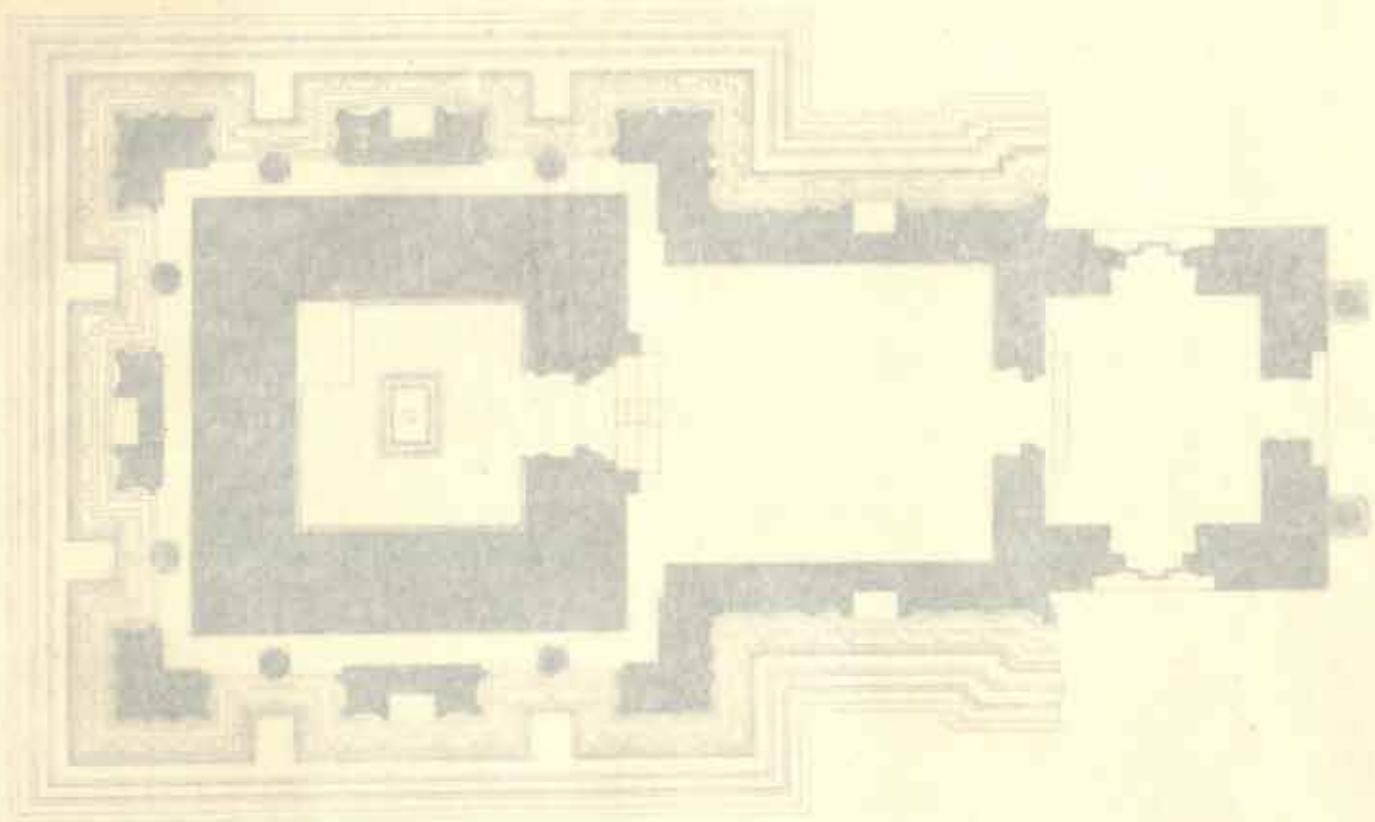
102. PLAN OF THE TEMPLE AT THIRUVALLI (MIRAMBAKKU) SCALE 1/4" TO 1'
