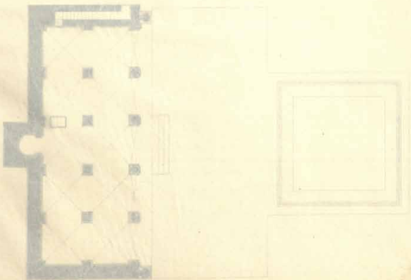
101. PLAN OF THE JAM' MASJID AT BILALA (MOKKAPATA) SCALE 1/4" TO 1'
